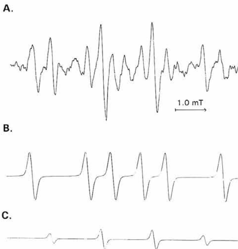
FIGURE 3 DMPO-OH and DMPO-hydroxyethyl adducts obtained at pH 3-3.5 after addition of H_2O_2 to the supernatant fluid of LPS-stimulated macrophages containing ethanol (1.7 M). (A) Experimental EPR spectrum; (B) EPR computer simulation of the DMPO-hydroxyethyl adduct; (C) Computer generated difference between DMPO-OH EPR spectrum in (A) and in Figure 2B. Receiver gain: 1.25 \times 10^5 .
