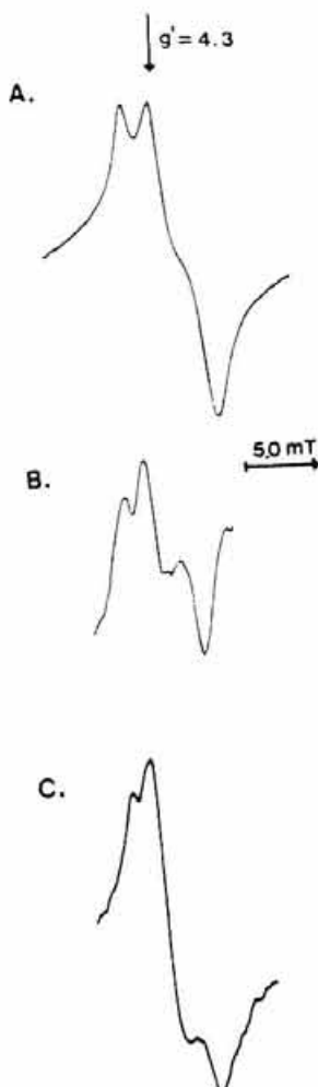
FIGURE 1 EPR spectra of lactoferrin recorded at 77^\circ \text{K} . (A) Lactoferrin (5 mM HEPES, pH 7.8); (B) Lactoferrin/NO mixture (5 mM HEPES, pH 7.8); (C) Lactoferrin in supernatant fluid after activation of macrophages (pH 7.9). Receiver gain: 1.25 \times 10^3 for A; 5 \times 10^3 for B; and 8 \times 10^4 for C.
